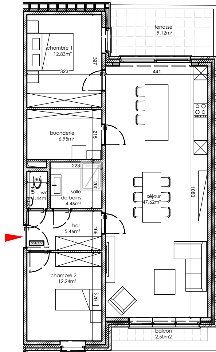
Plan Ech: 1/100
