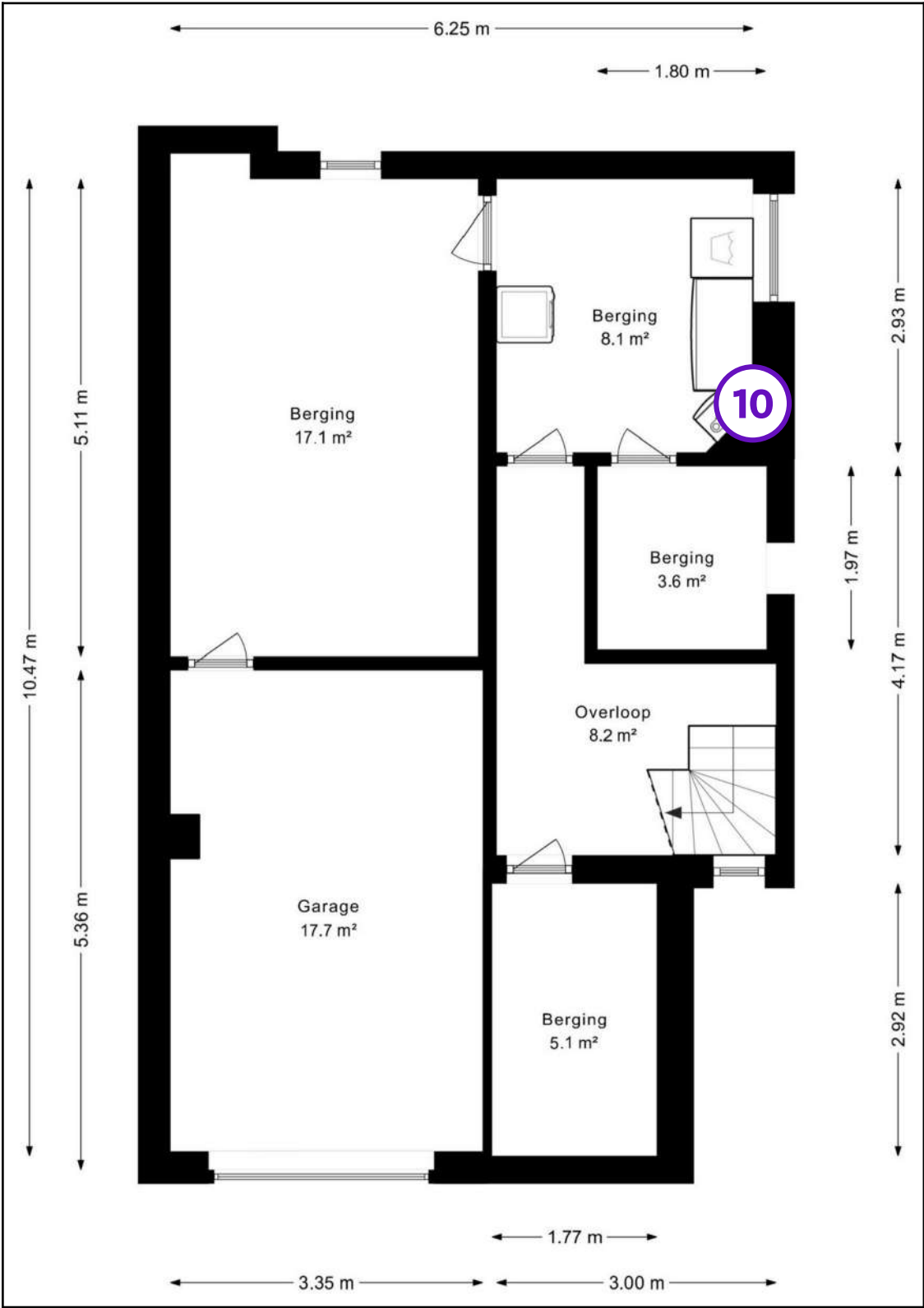
Legende van plan 1.13: Garage
