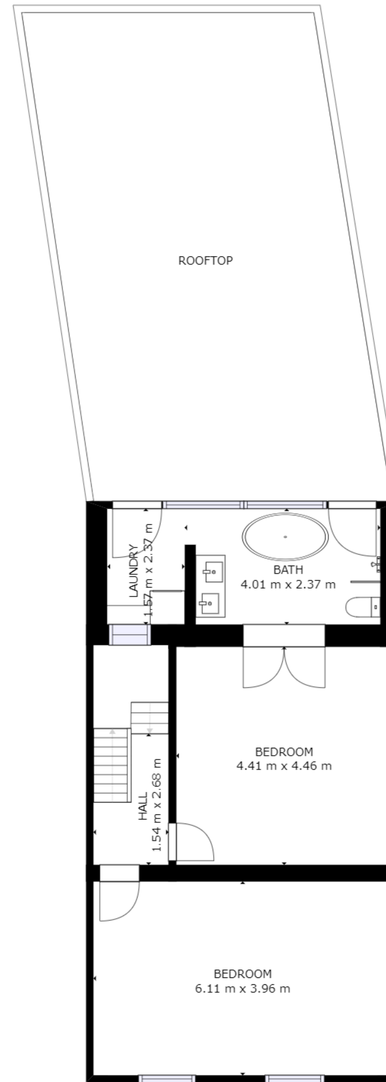
FLOOR 2
