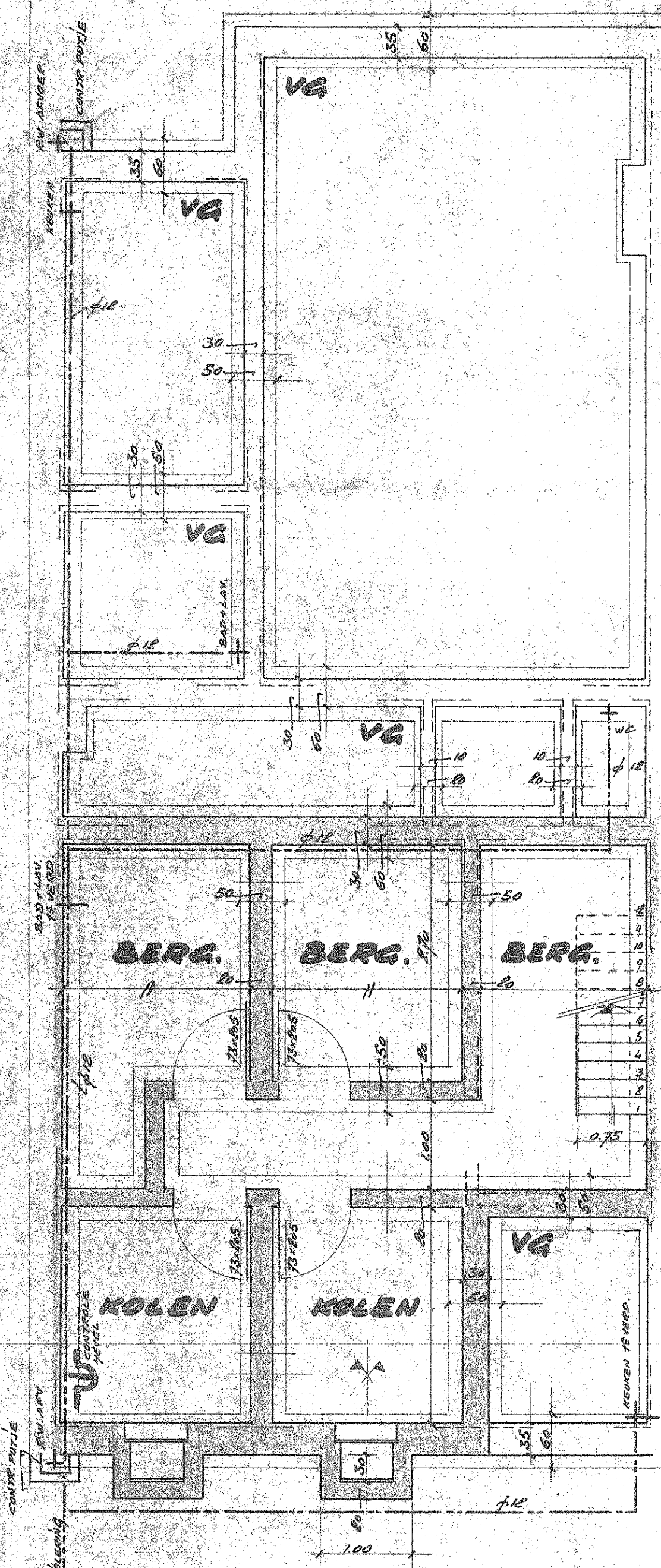
KELDER-FUNDERING-EN RIOLERINGSPLAN
