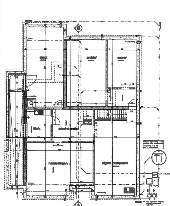
KELDER-FUNDERING-RIOLERING
