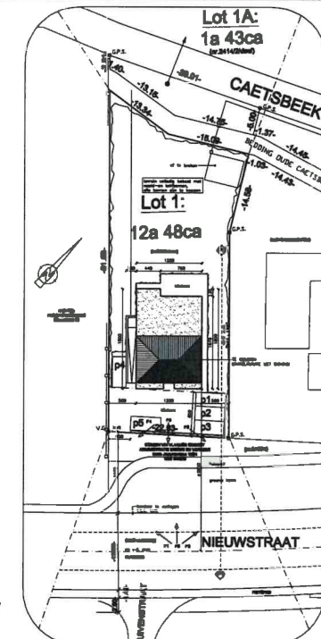
INPLANTING 1/250
