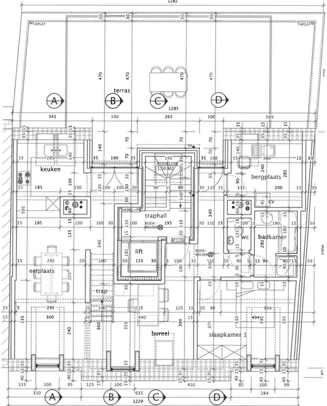
ZOLDERPLAN schaal 1/50
