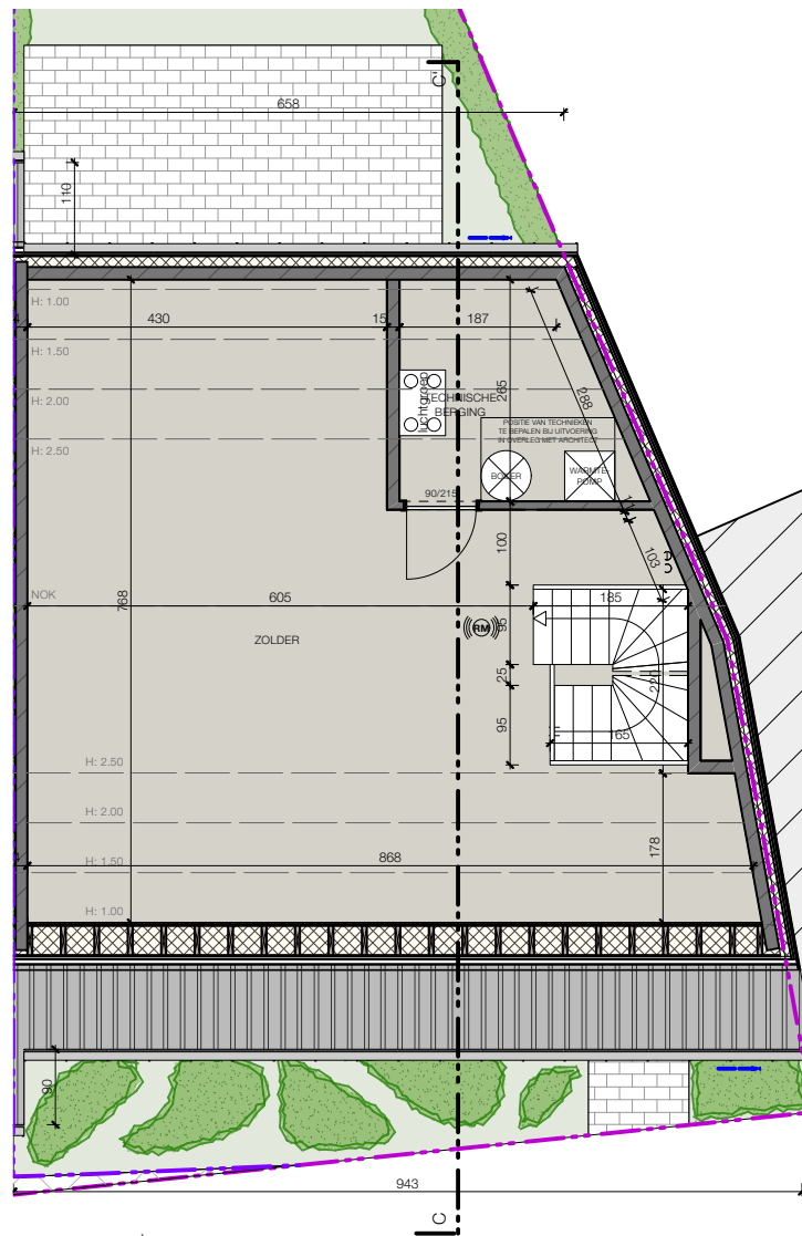
2° VERDIEPING WONING 4 Bruto: 69,96 m 2
