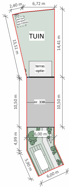
INPLANTINGSPLAN 1:500
