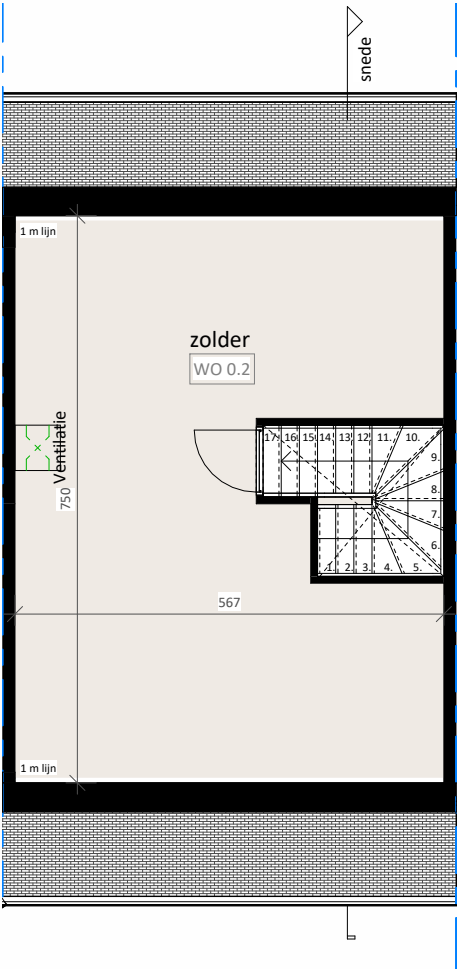
ZOLDER 1:100
