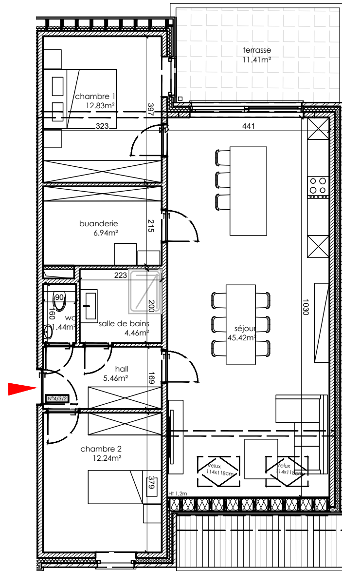
Plan Ech: 1/100
